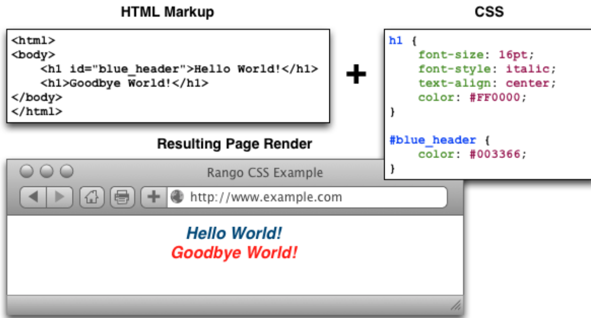
Fig. 19.2: An illustration demonstrating the use of an id selector in CSS. Note the blue header has an identifier which matches the CSS attribute #blue_header .
