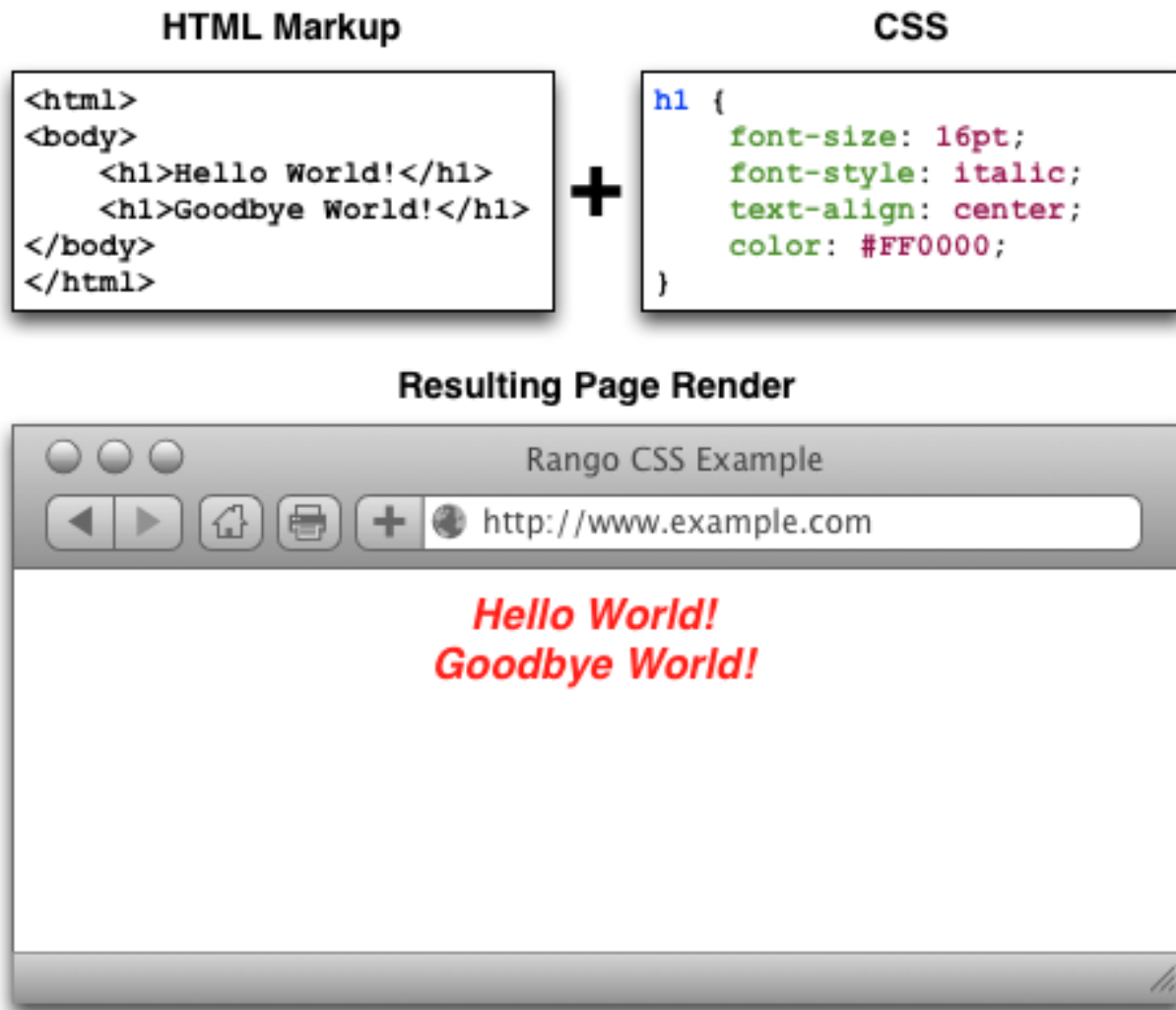
Fig. 19.1: Illustration demonstrating the rendered output of the sample HTML markup and CSS stylesheet shown. Pay particular attention to the CSS example - the colours are used to demonstrate the syntax used to define styles and the property/value pairings associated with them.
