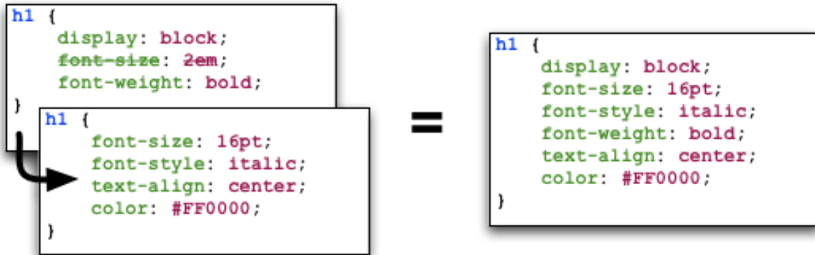
Fig. 19.7: Illustration demonstrating the cascading in Cascading Style Sheets at work. Take note of the font-size property in our h1 style - it is overridden from the default value. The cascading styles produce the resultant style, shown on the right of the illustration.
