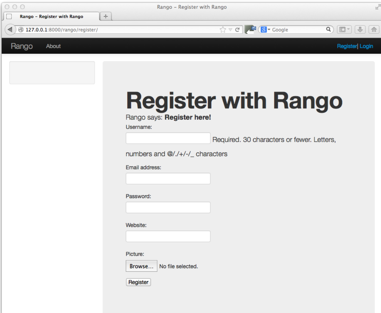
Fig. 11.3: A screenshot of the Registration page with Bootstrap Styling applied but not customised.
