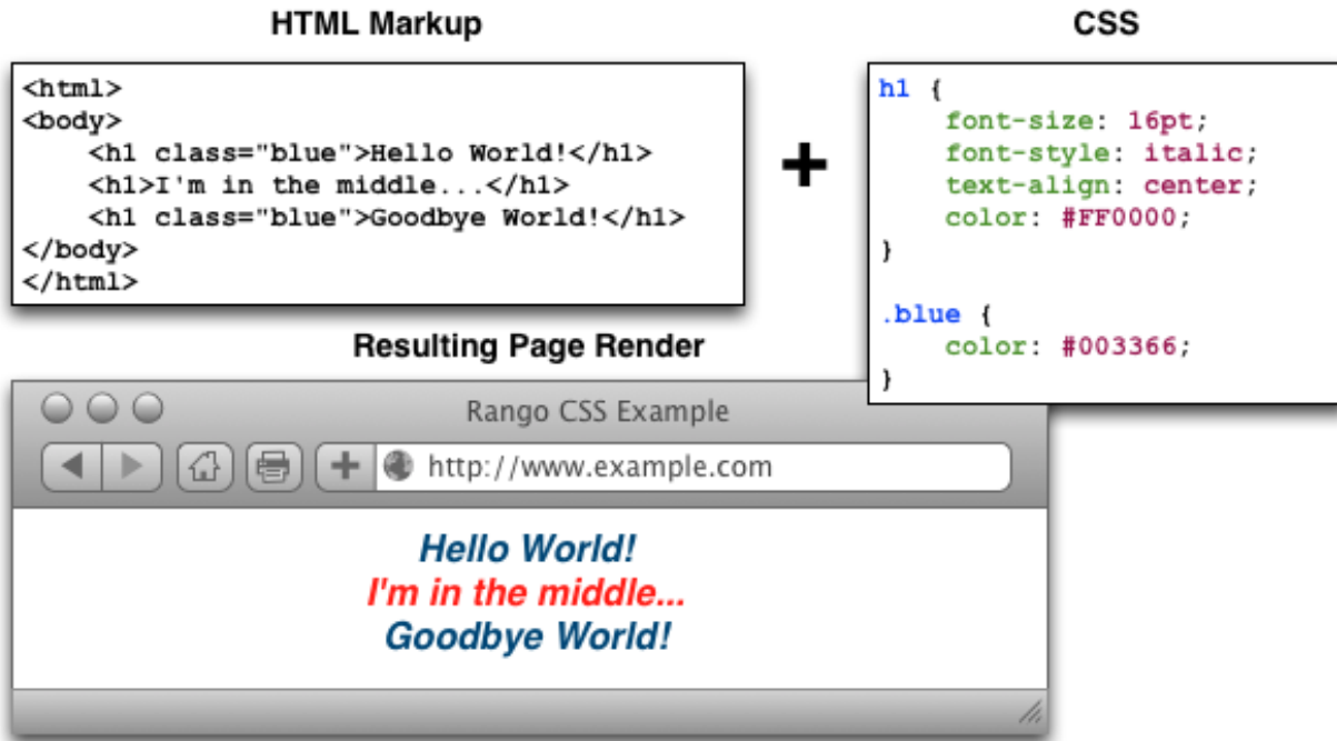
Fig. 19.3: An illustration demonstrating the use of a class selector in CSS. The blue headers employ the use of the .blue CSS style to override the red text of the h1 style.
